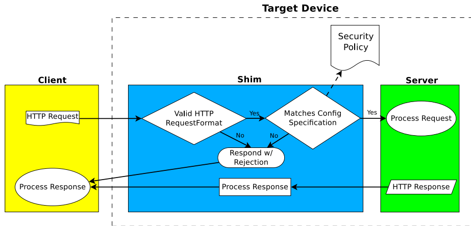
Figure 1. Umbra Architecture —A lightweight software “shim” runs on the embedded device and transparently proxies client requests, rejecting those that are malformed or that do not match a predefined security policy.
