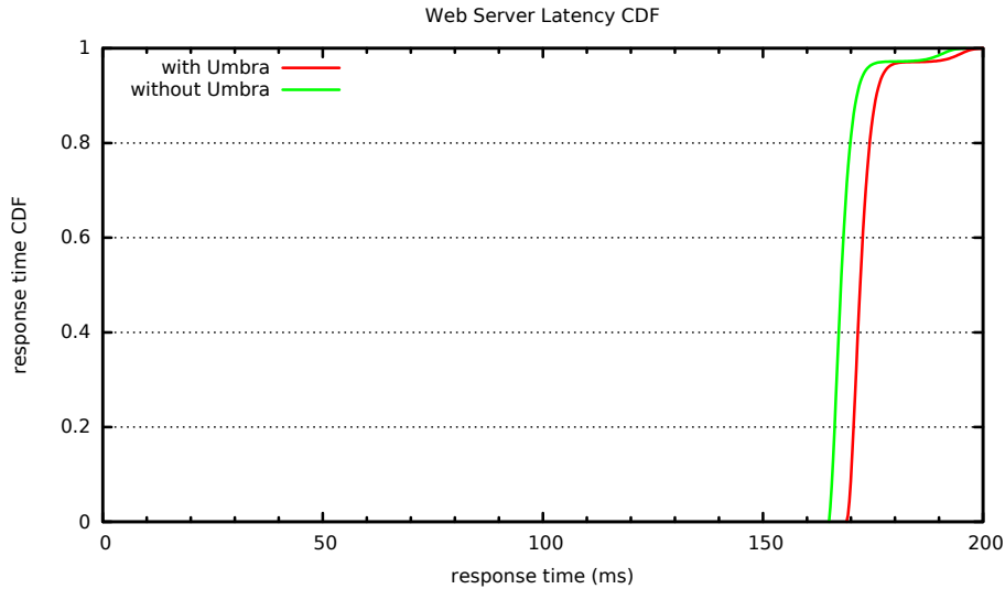
Figure 3. Server Response Time —This graph shows the response time of the web server with and without Umbra; the average overhead is about 5 ms (3%).
